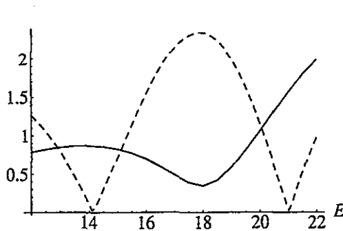
Figure 4. Absolute values of \zeta(s) (dashed curve) and the Gauss map eigenfunction h_s(0.5) (computed from the integral (35)) (full curve) on the critical line s=1/2+iE .
