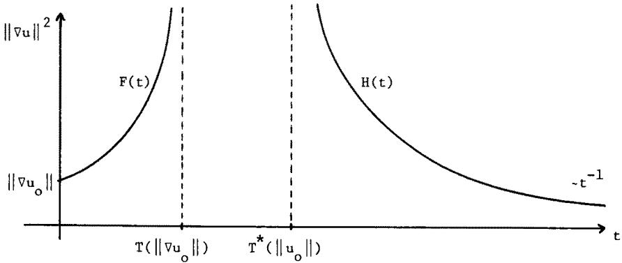
Figure 1. Estimates (16) and (35) for the Galerkin approximations.
