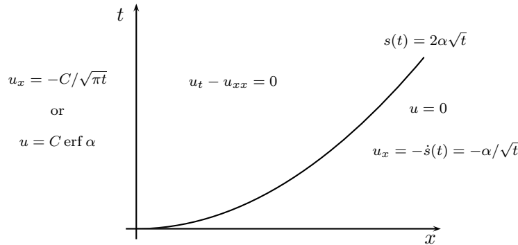
FIGURE 2. The Stefan problem solved by u in (3.1)
